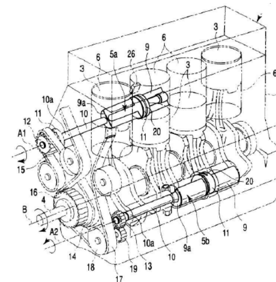
CN1297762C - Balance shaft and engine
